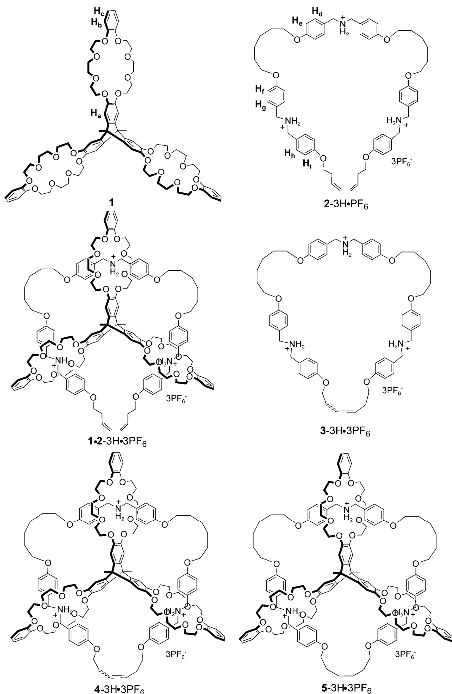
Scheme 1. Structures and proton designations of host 1 , trisdialkylammonium strand 2-3H•PF 6 , [2](3)pseudorotaxane 1-2-3H•3PF 6 , trisdialkylammonium macrocycle 3-3H•PF 6 , and [2](3)catenanes 4-3H•3PF 6 and 5-3H•3PF 6 .
