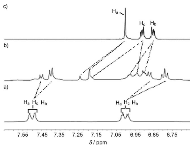
Figure 1. Partial ^1\text{H} NMR spectra (600 MHz, [\text{D}_6]\text{acetone} ) of a) 2\text{-}3\text{H}\cdot 3\text{PF}_6 (1.0 mm) at 228 K, b) 1 (1.0 mm) and 1 equiv of 2\text{-}3\text{H}\cdot 3\text{PF}_6 at 228 K, and c) host 1 (1.0 mm) at 228 K. Resonance protons are labeled in Scheme 1.
